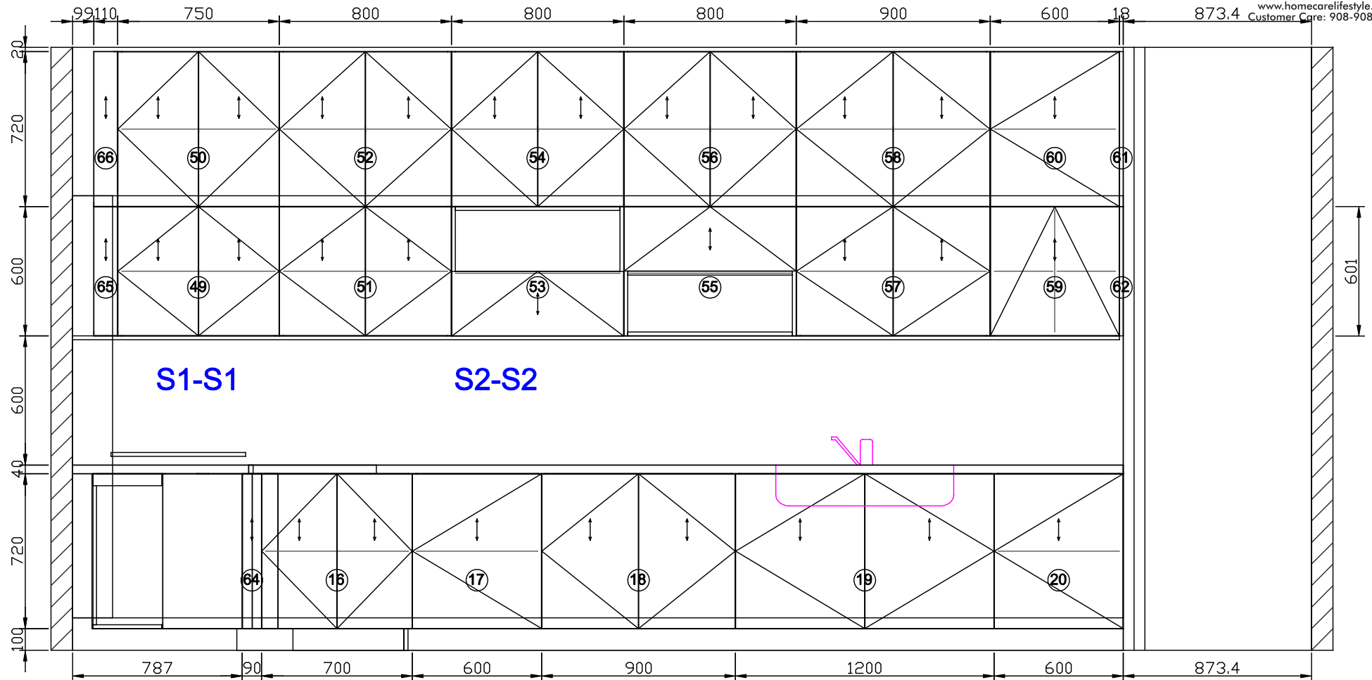
C View elevation drawing
